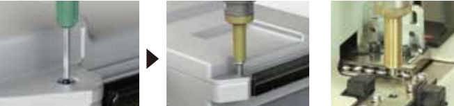
One system can apply screw lock adhesive and tighten screws With screw feeder
